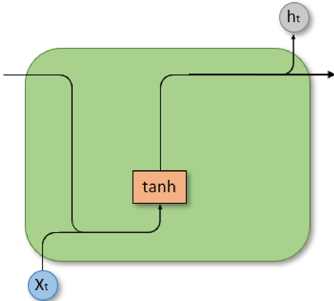
RNN
