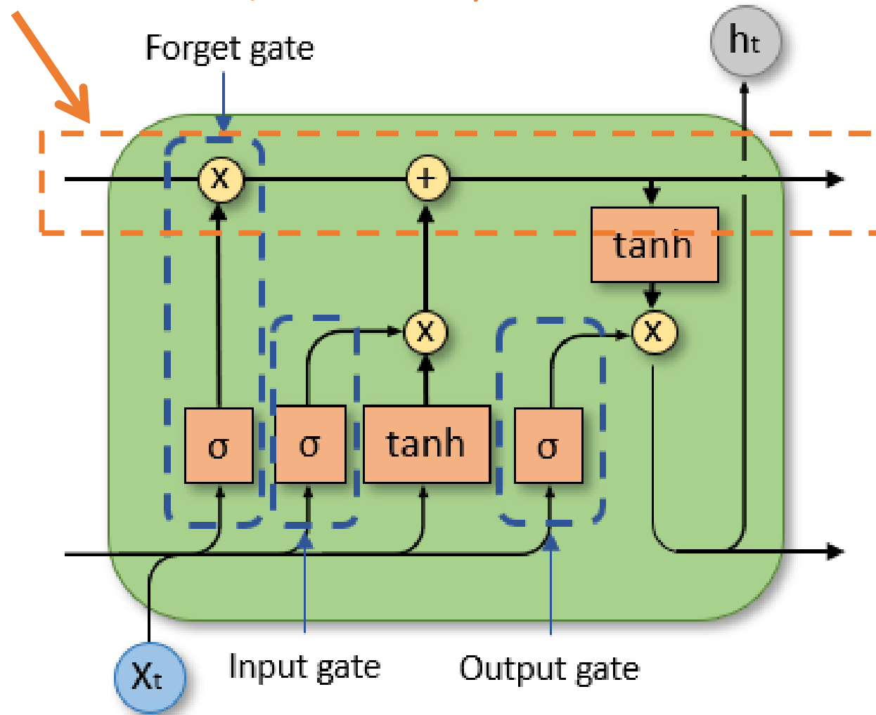
LSTM
